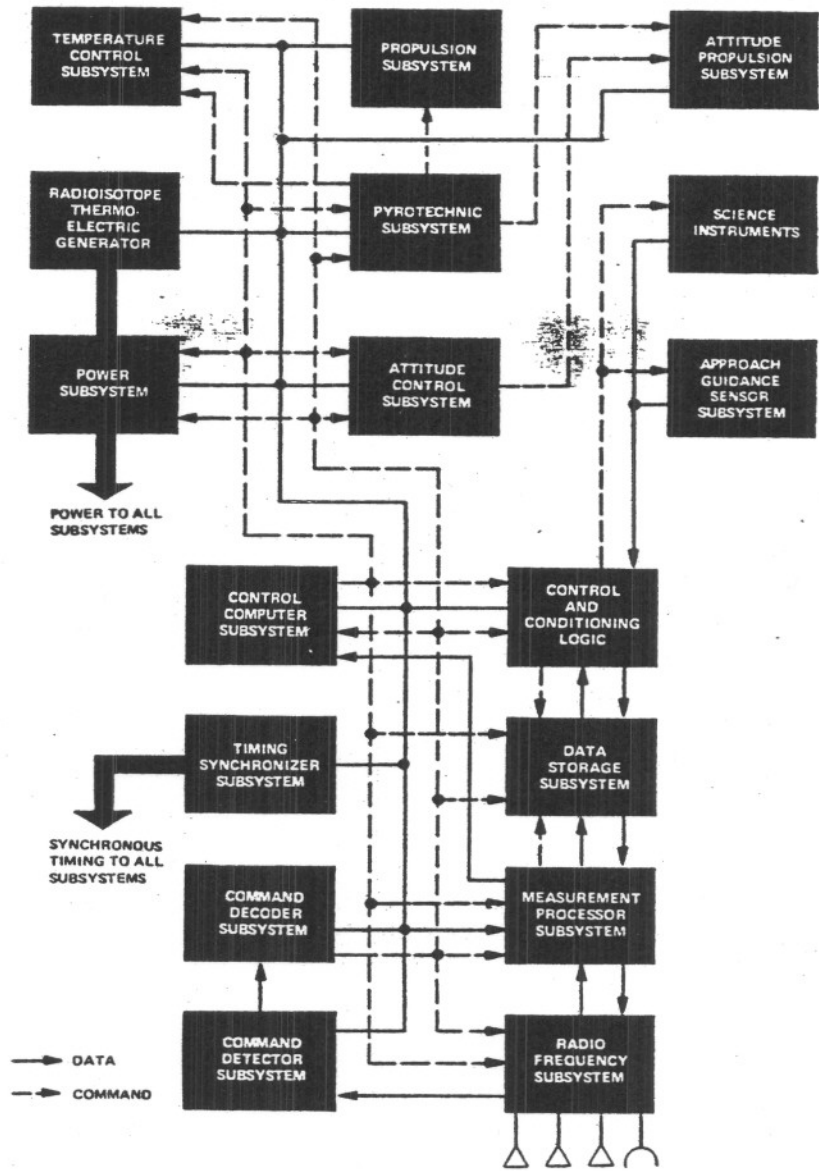
TOPS FUNCTIONAL BLOCK DIAGRAM
