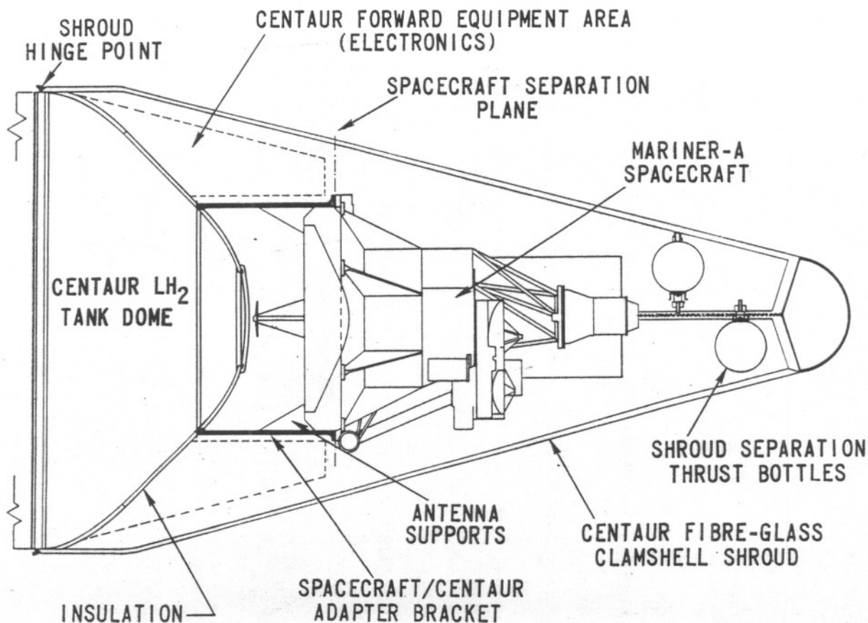
Mounting of Mariner in Centaur Nose Cone
