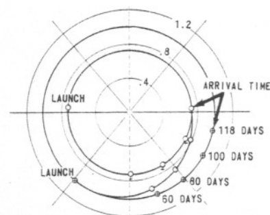
Mariner Flight to Venus
